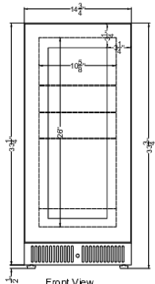
Front View
