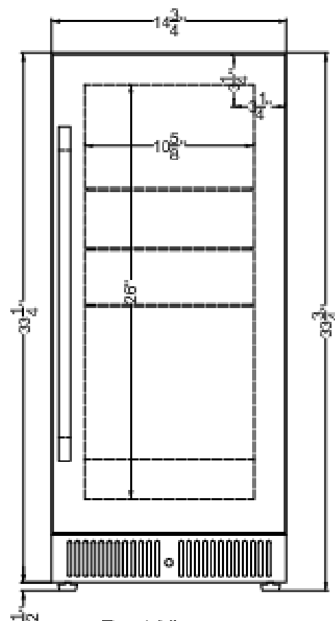
Front View
